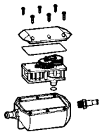
HYDRO TIMER
