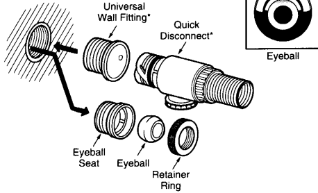
Eyeball Fitting Connection Kit (part #9-100-8001)
