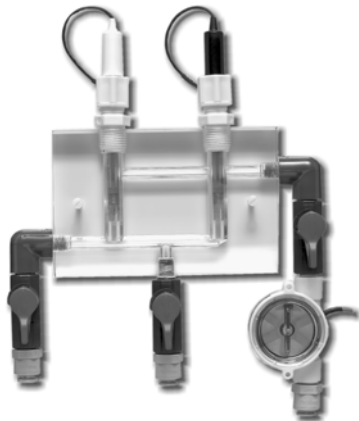
V4628 Flow Cell w/Rotary Sensor
