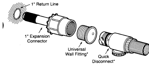
1" Stub Pipe Connection Kit (part #9-100-8002)
