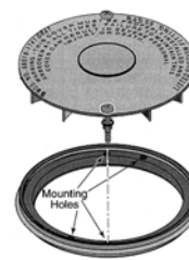
Swimquip Anti-Vortex Grate
