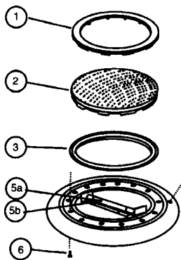
Light Assembly
